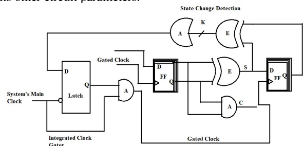
Fig 1. Data Driven Clock Gating
