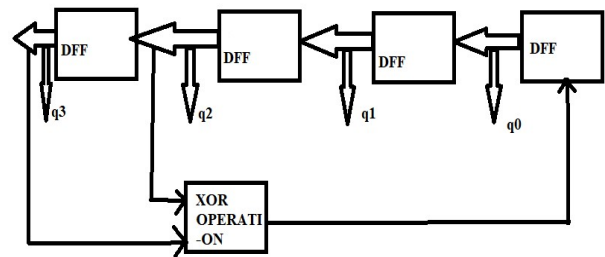
Fig 3. Schematic of LFSR without LACG Technique
