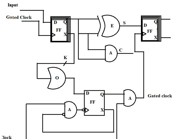
Fig 2. Look Ahead Clock Gating
