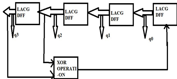
Fig 4. Schematic of LFSR with LACG Technique
