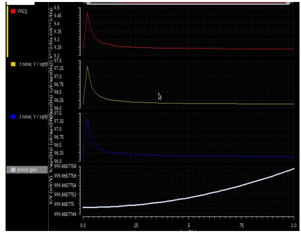
Fig 7. Noise Response of Data driven Clock Gating
