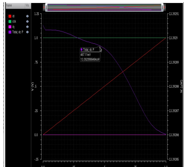
Fig 9. Power Response of Look Ahead Clock Gating
