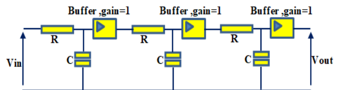
Figure10. Simulation of the 3rd order delayed system
