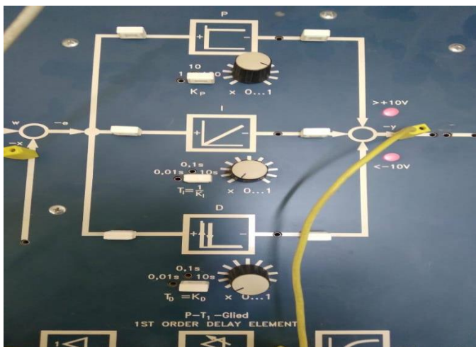
Figure8. PID controller
