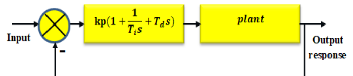
Figure 1. Closed-loop system
