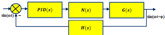
Figure13. Closed loop structure of nonlinear with sinusoidal input
