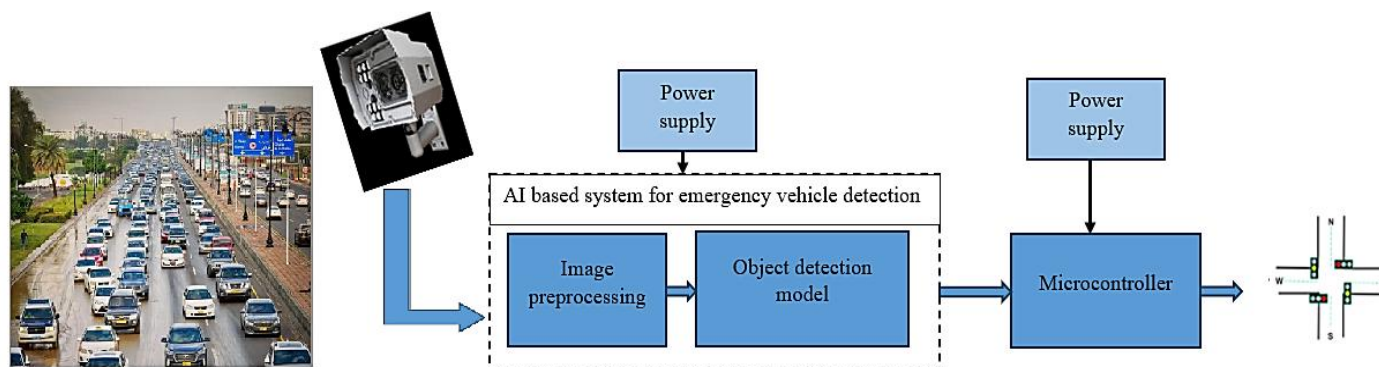
Figure 1. Proposed system process-flow diagram
