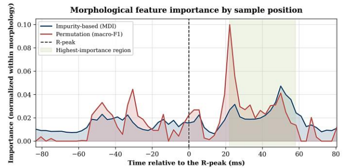
Figure 6. Morphological feature importance by sample position relative to the R-peak, by both methods
