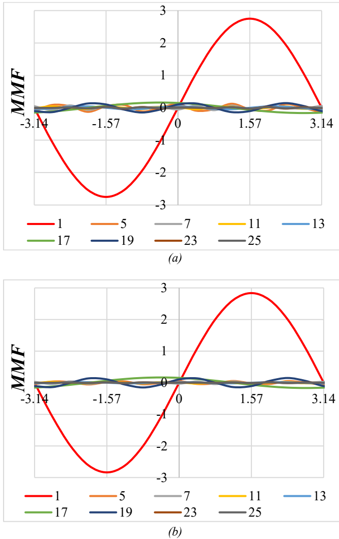
Figure 3. Spatial MMF harmonic spectrum obtained by DFT analysis: standard; (b) combined
