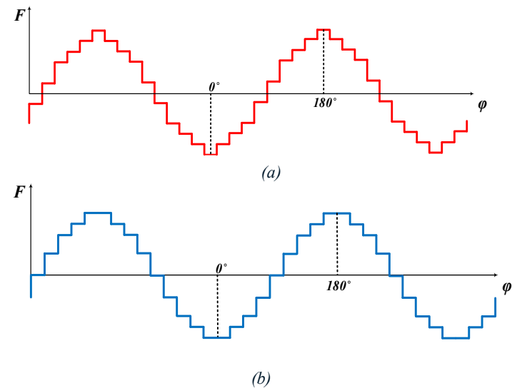
Figure 2. MMF distribution curve for a single-layer winding with Z=36 , p=2 , y=9 : (a) standard winding; (b) combined winding
