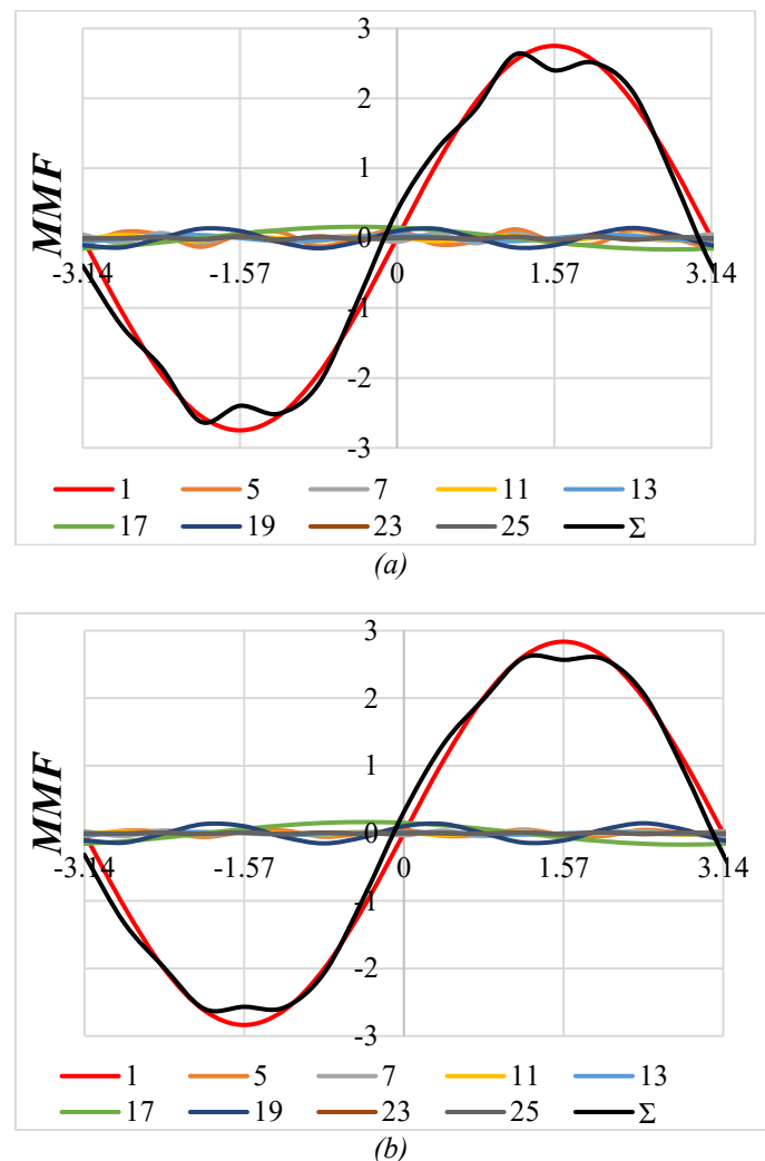
Figure 4. Spatial MMF harmonic spectrum obtained by DFT analysis: standard; (b) combined
