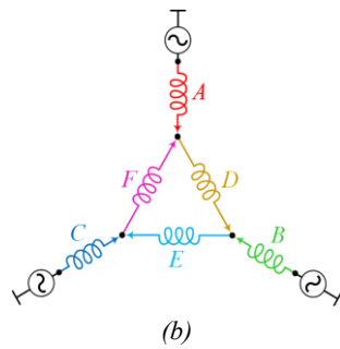
Figure 1. Basic circuit scheme of the combined winding: (a) parallel; (b) series
