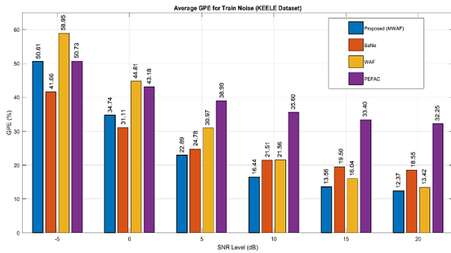
Figure 4. Average Gross Pitch Error (GPE) Rate for Train Noise in KEELE Database
