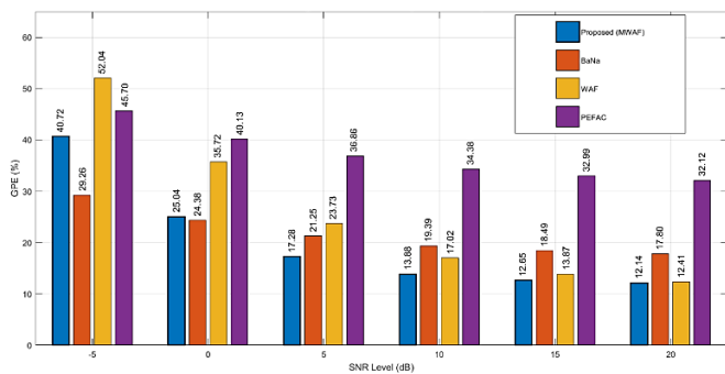
Figure 5. Average Gross Pitch Error (GPE) Rate for HF Channel Noise in KEELE Database
