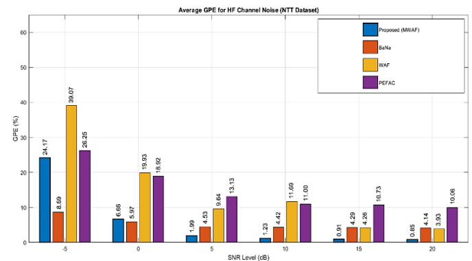
Figure 9. Average Gross Pitch Error (GPE) Rate for HF Channel Noise in NTT Database
