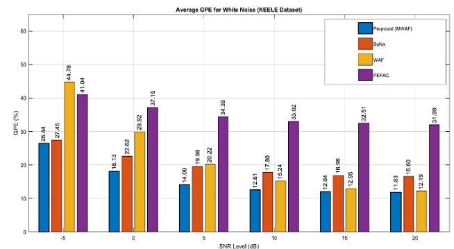
Figure 2. Average Gross Pitch Error (GPE) Rate for White Noise in KEELE Database
