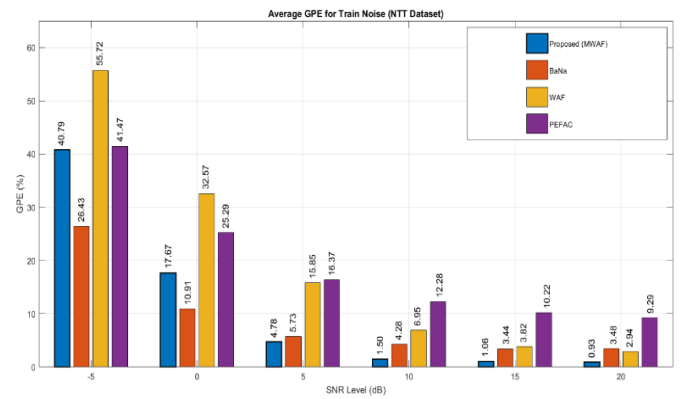
Figure 8. Average Gross Pitch Error (GPE) Rate for Train Noise in NTT Database
