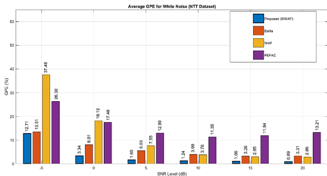
Figure 6. Average Gross Pitch Error (GPE) Rate for White Noise in NTT Database
