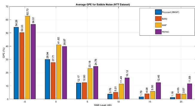
Figure 7. Average Gross Pitch Error (GPE) Rate for Babble Noise in NTT Database
