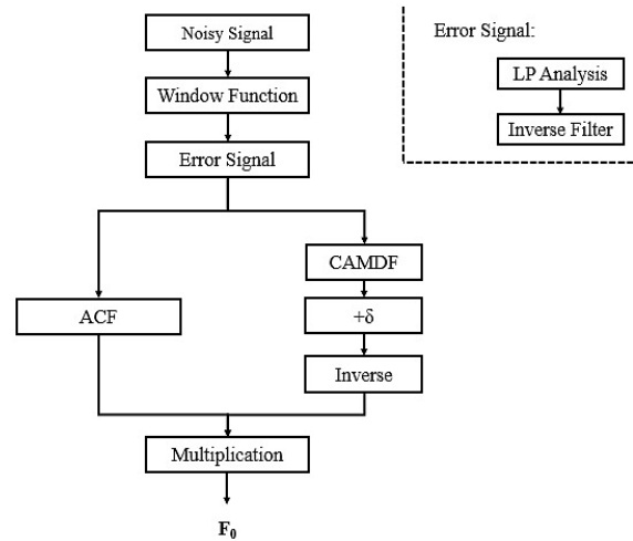
Figure 1. Block diagram of the proposed method
