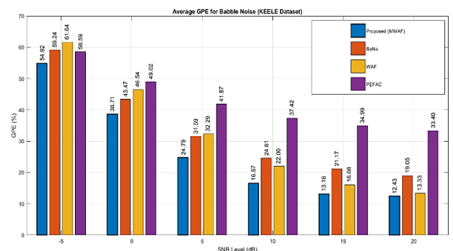
Figure 3. Average Gross Pitch Error (GPE) Rate for Babble Noise in KEELE Database
